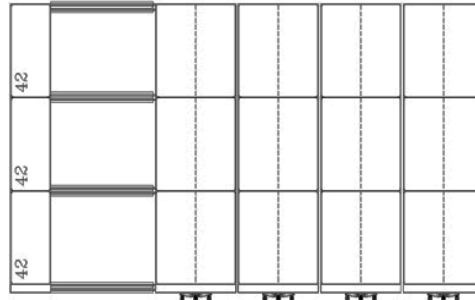
Mobile Aisle System with 42" Roll Out Drawers 4,808 letter filing inches 205 sq. ft. required
